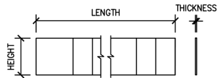
B 9 SIERRA SHAKE SIDING DIMENSIONS NOT-TO-SCALE
