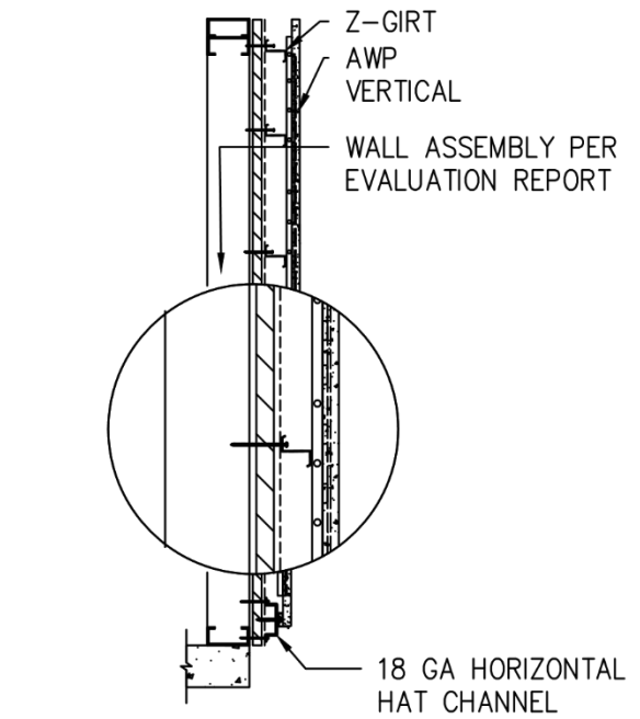
STEEL STUDS W/ HORZ. Z-GIRT
