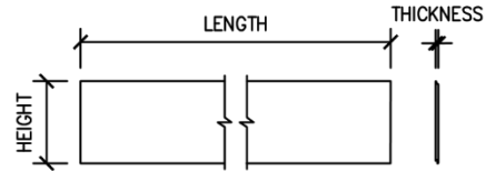
C 9 AWP SIDING DIMENSIONS NOT-TO-SCALE
