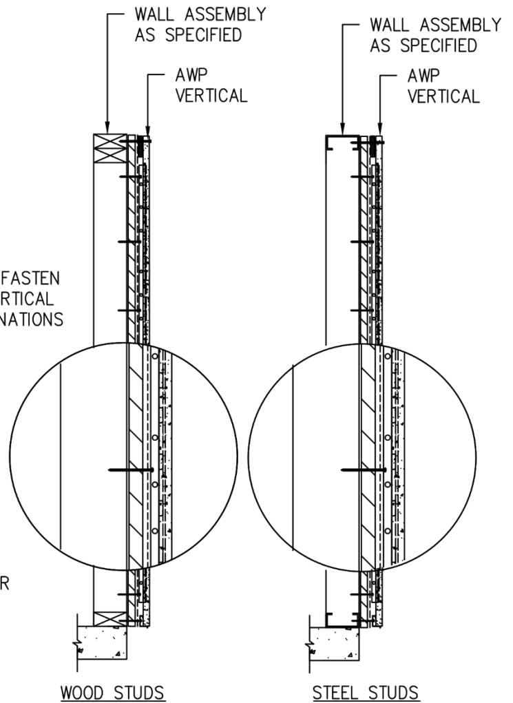
A 2 AWP VERT. INSTALL INTO WOOD OR STEEL STUDS ELEVATION VIEW NOT-TO-SCALE B 2 AWP VERT. INSTALL INTO WOOD OR STEEL STUDS SECTION VIEW NOT-TO-SCALE
