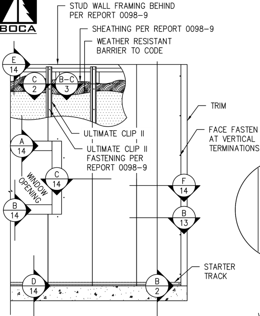
A 2 AWP VERT. INSTALL INTO WOOD OR STEEL STUDS ELEVATION VIEW NOT-TO-SCALE B 2 AWP VERT. INSTALL INTO WOOD OR STEEL STUDS SECTION VIEW NOT-TO-SCALE
