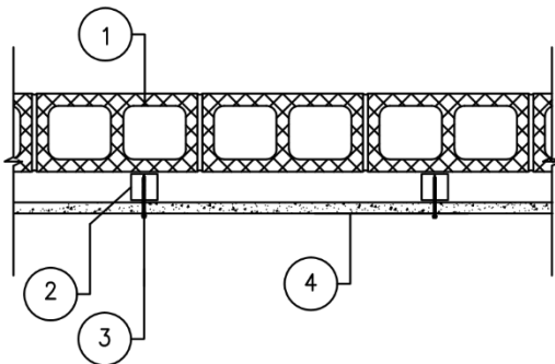
C 11 SIERRA/SAVANNAH INSTALL INTO WOOD FURRING AND CONCRETE PLAN VIEW NOT-TO-SCALE NOTE: 1. FURRING FASTENING NOT SHOWN FOR CLARITY
